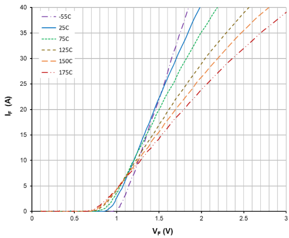
Figure 1. Forward Characteristics
