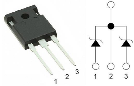
TO-247-3
