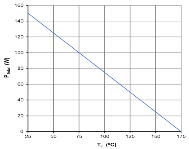
Figure 4. Power Derating
