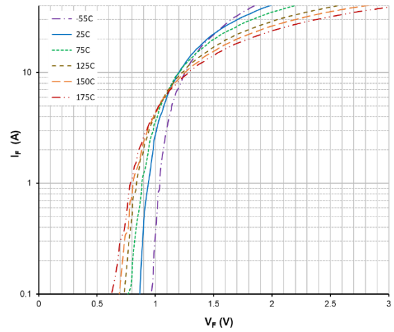
Figure 2. Forward Characteristics
